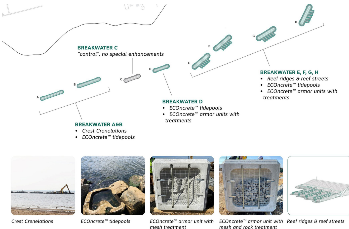
Figure 4A.3 Diagram of the Living Breakwaters project in Staten Island, New York, demarcating the various types of units used to retrofit the breakwaters. Diagram and photos courtesy of Kate Orff.
